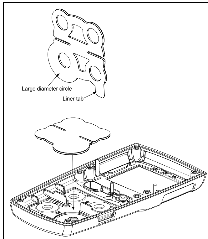
Figure 10. Liner Tab
