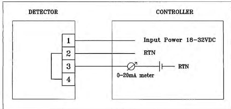
Figure 13: 0-20mA Non-Isolated Sink 3-Wire
