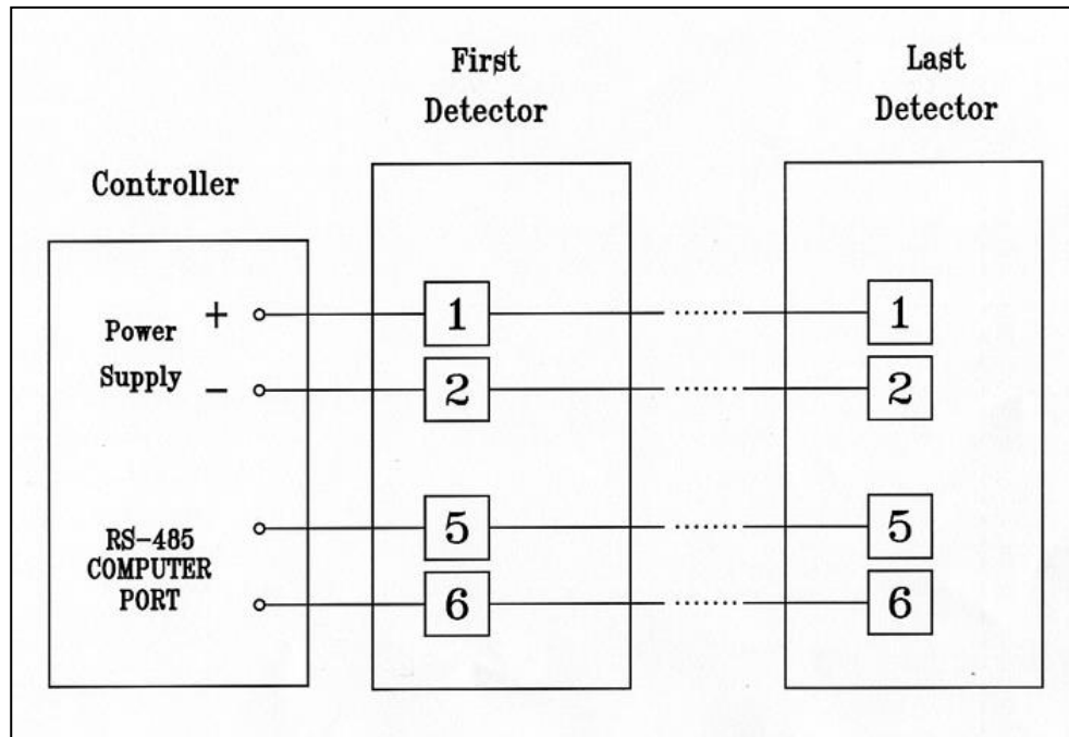
Figure 15: RS-485 Networking for Wiring Option 3
